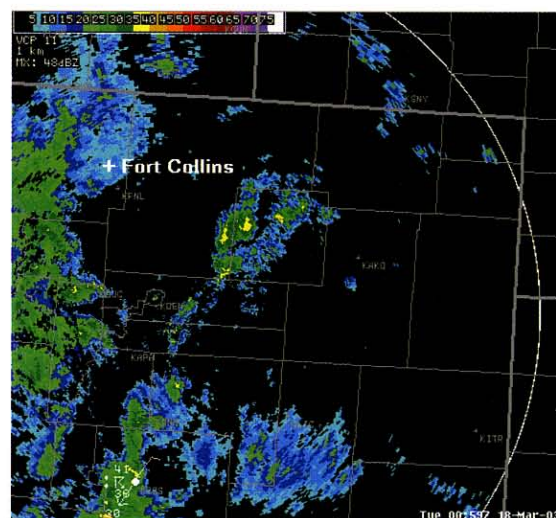
Figure 4. One line of convection moves off to the west of Fort Collins (squall lines were moving westward) as a second line forms to the east. Figure shows the 0.5 degree tilt, PPI reflectivity scan taken from the Denver, Colorado WSR-88D at around 6:00 pm on the evening of 17 March 2003.
