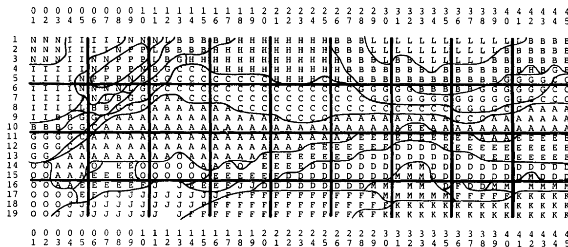
FIG. 8. Blocks for "operational" 5 \times 5 grouping of VAS FOVs shown over clusters from Fig. 7.
