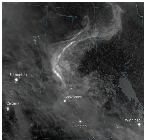
FIG. 10. VIIRS DNB image of the aurora borealis over central Canada from 0916 UTC 9 Mar 2012. Canadian provincial boundaries are shown with Saskatchewan in the middle of the image. With a full moon on 8 Mar 2012, clouds, snow, and ice-covered lakes are visible, along with city lights. Lights from major cities in the region have been labeled. The aurora extends from west-central Saskatchewan to northwestern Manitoba.
