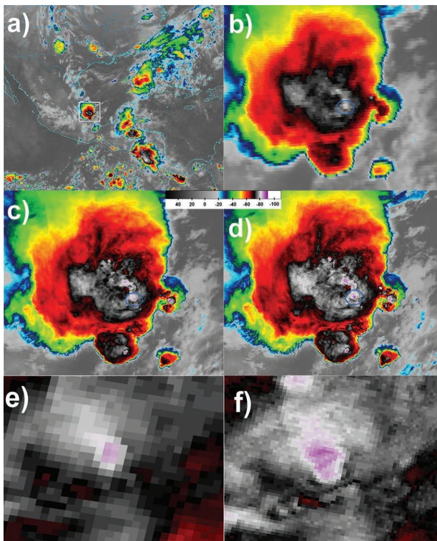
FIG. 2. (a) GOES-13 10.7\text{-}\mu\text{m} image from 0815 UTC 6 Jun 2012, (b) zoomed-in version of (a) over the highlighted thunderstorm complex in the southwestern Gulf of Mexico, (c) Aqua MODIS band 31 ( 11.0\text{ }\mu\text{m} ) view of the same thunderstorm complex at 0816 UTC, and (d) NPP VIIRS band I5 ( 11.45\text{ }\mu\text{m} ) view at 0817 UTC. An extreme close-up approximately covering the circled region from the MODIS image in (c) is shown in (e), and a similar close-up from VIIRS is shown in (f). The legend shows the brightness temperatures ( ^{\circ}\text{C} ).
