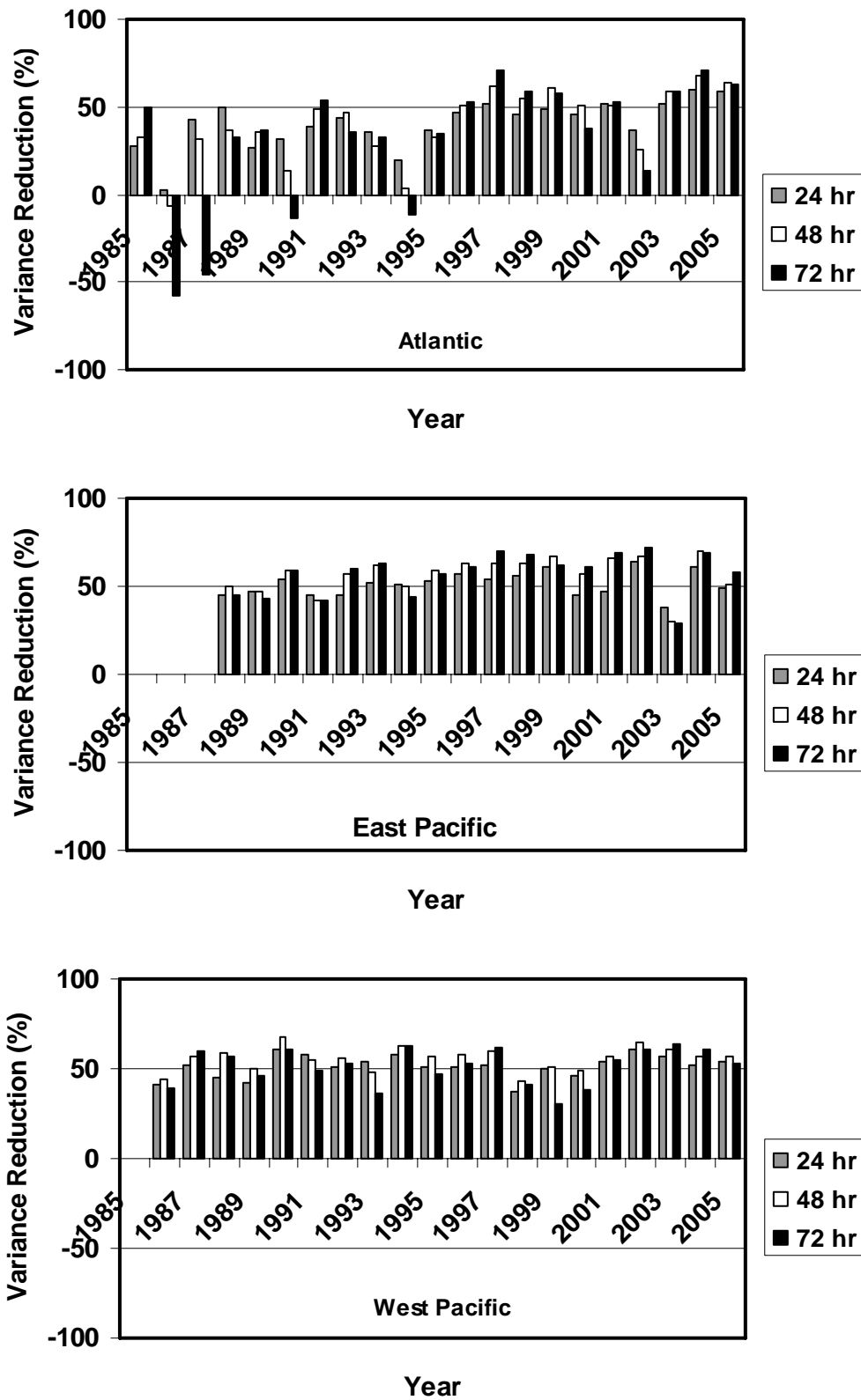
Figure 2. The time evolution of the intensity variance reduction due to the NHC or JTWC forecasts.
