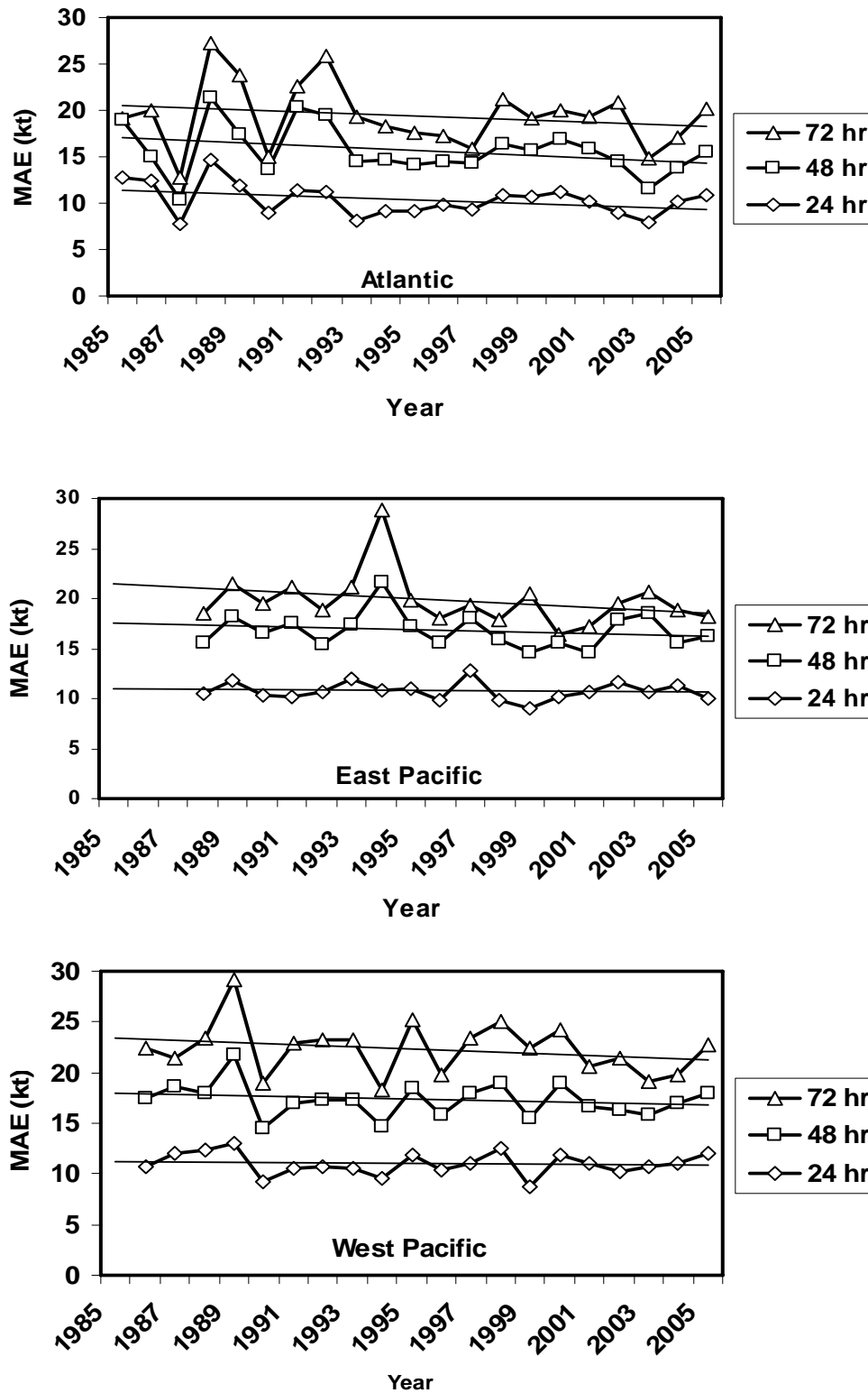
Figure 1. The time evolution of the mean absolute error of operational intensity forecasts with linear trend lines.
