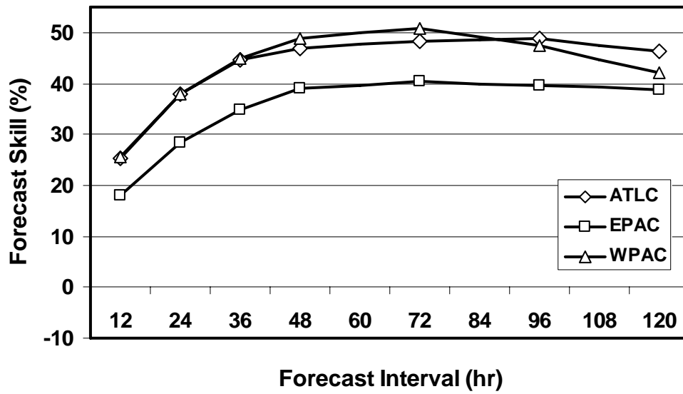
Figure 5. The skill of the NHC (ATLC and EPAC) or JTWC (WPAC) track forecasts for 2001-2005.
