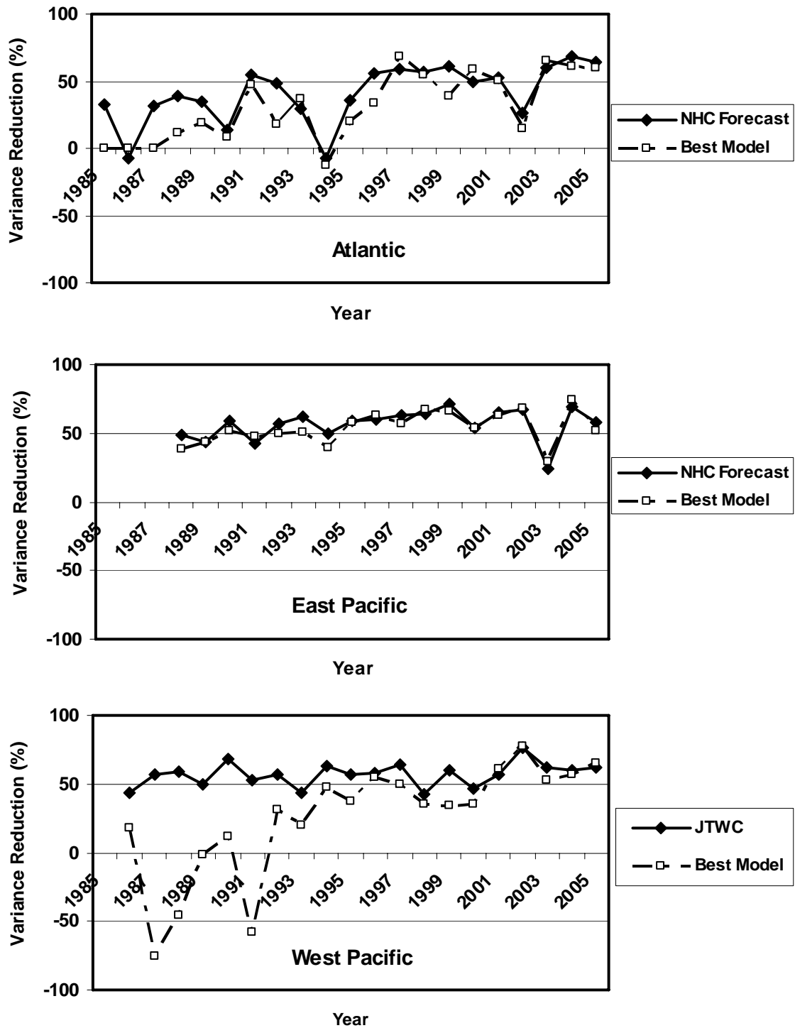
Figure 3. The time evolution of the variance reduction of the NHC or JTWC official 48 hr intensity forecast and that from the best guidance model.
