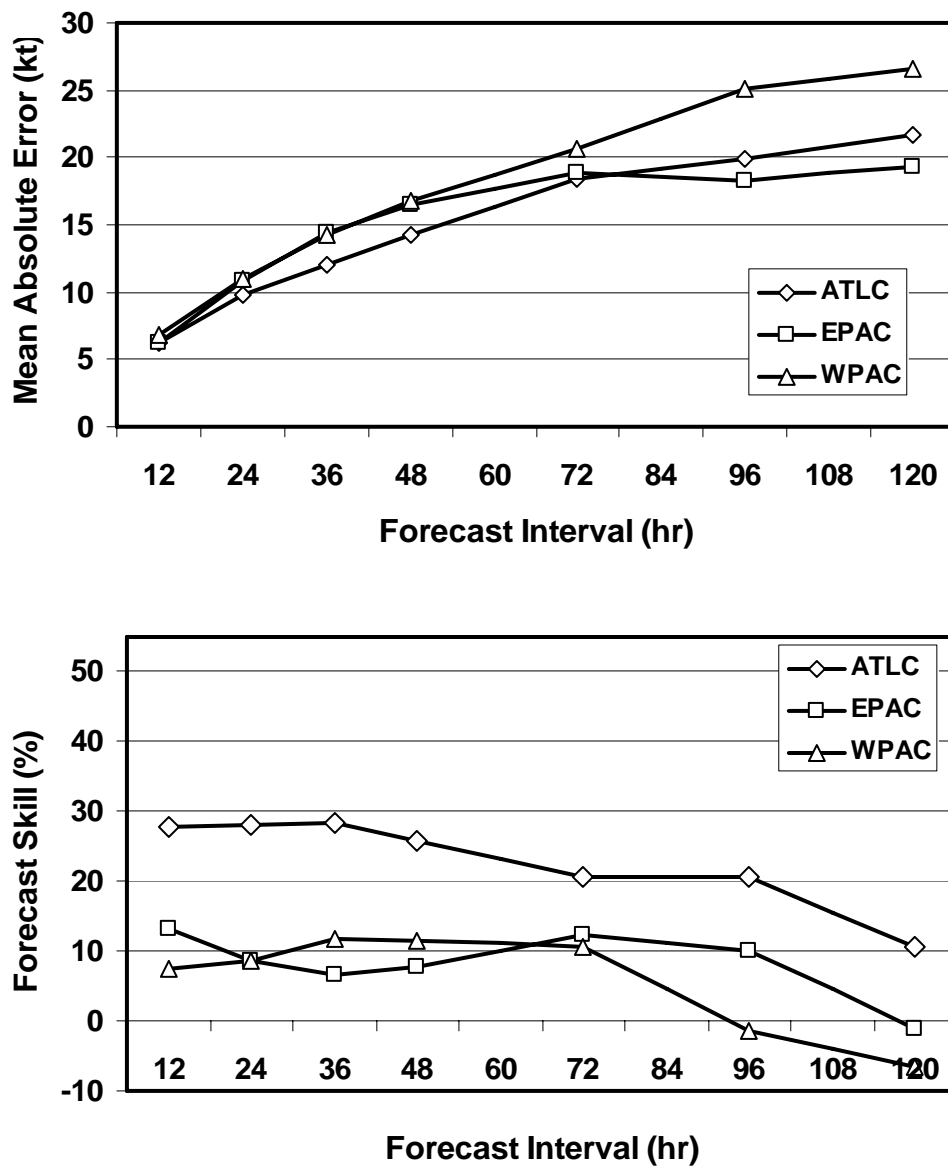
Figure 4. The mean absolute error of the 2001-2005 NHC or JTWC intensity forecasts for the Atlantic, East Pacific and West Pacific (upper) and the corresponding forecast skill (lower).
