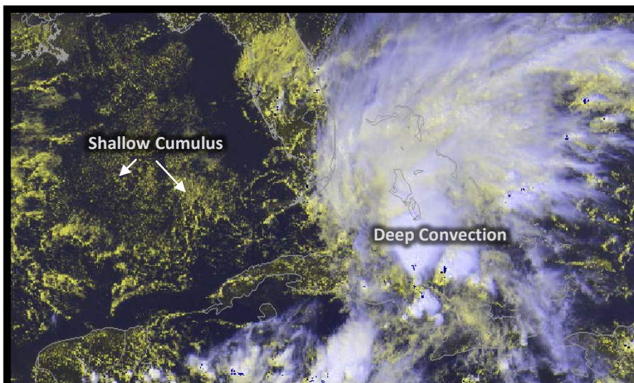
Day Cloud Convection RGB from GOES-16 ABI at 1857 UTC, 04 October 2017
