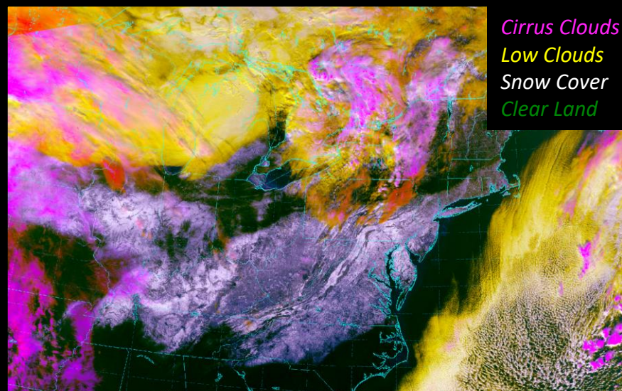
Daytime image of the Snow/Cloud Discriminator from S-NPP VIIRS over the mid-atlantic states at 1808 UTC, 24 January, 2016
