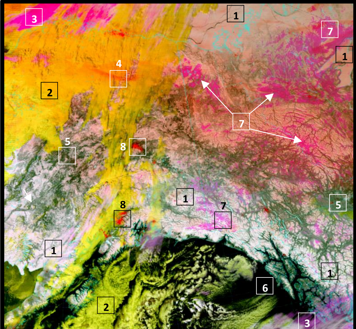
Nighttime image of Snow/Cloud Discriminator from S-NPP VIIRS over Alaska at 1121 UTC, 11 March 2017.
